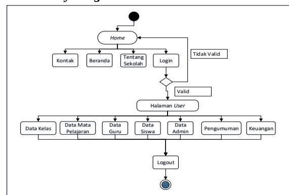
Gambar 3 Activity Diagram Admin
