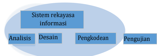
Gambar 1 Model WaterFall
