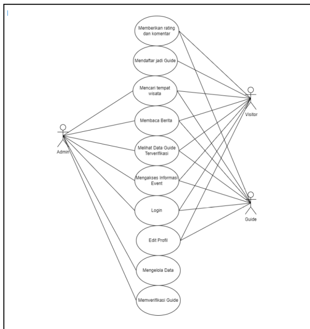
Gbr. 2 Use-case Diagram
